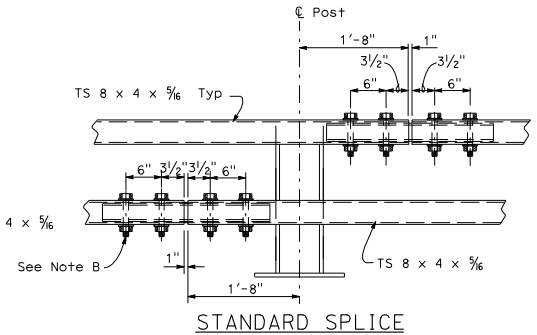
STANDARD SPLICE
