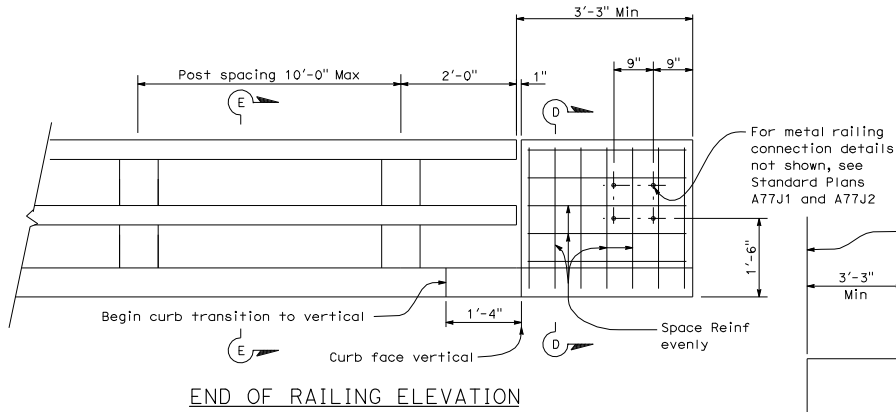
END OF RAILING ELEVATION
