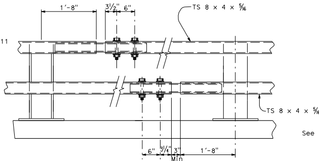
EXPANSION SPLICE
