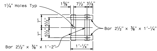
WALL ANCHOR PLATE DETAIL
